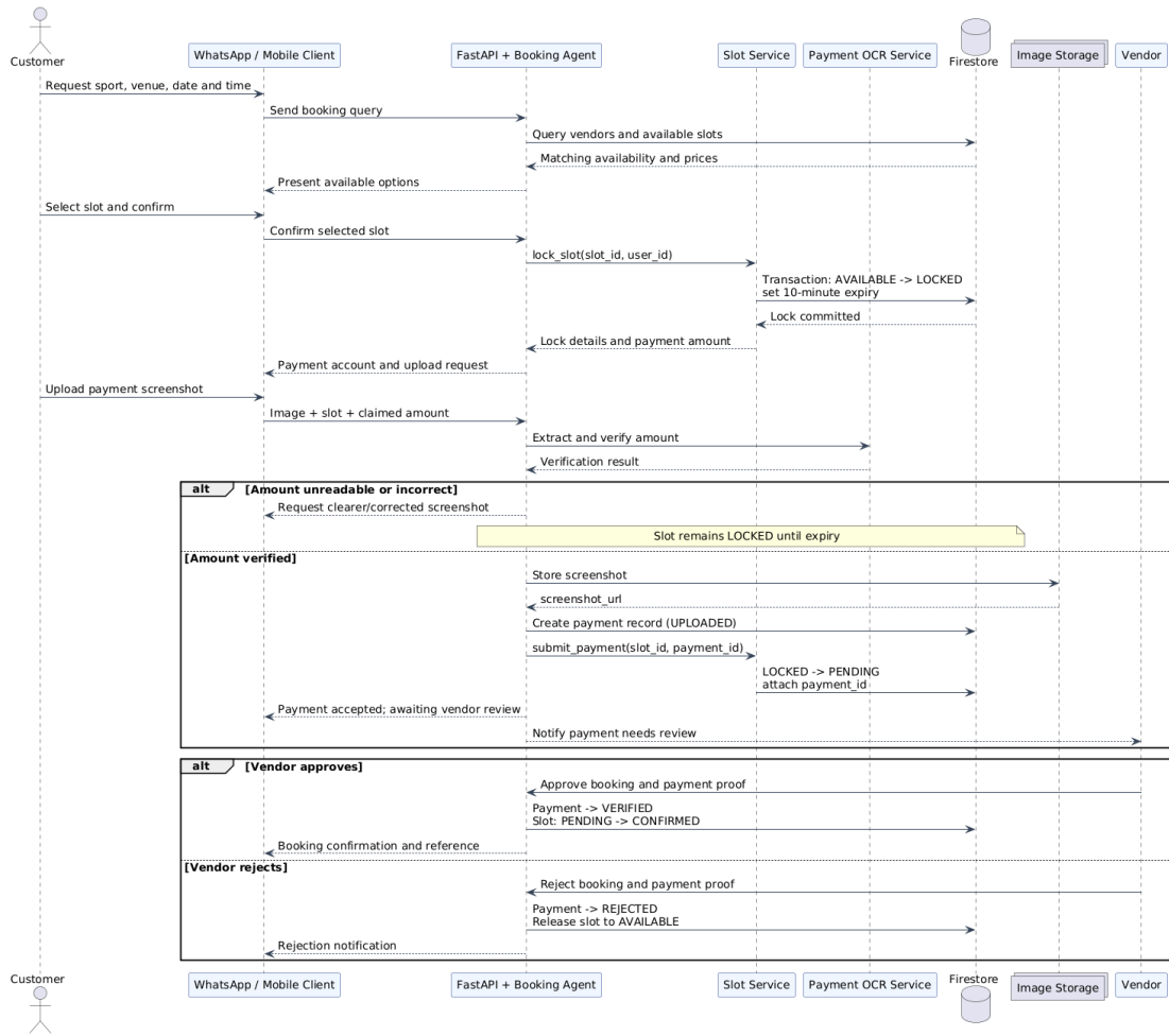
Figure 4.3: AI booking and payment sequence.
