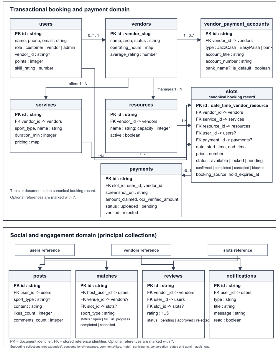
Figure 4.2: Core Firestore data model and payment relationships.
