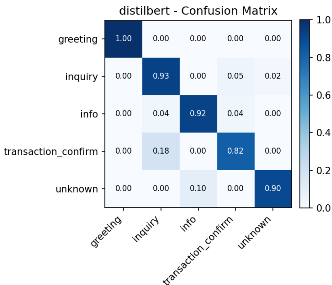
Figure 6.2: Confusion matrix for DistilBERT
